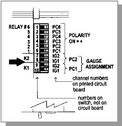
Figure 2-9 Partial Top View of Process Control Module.
