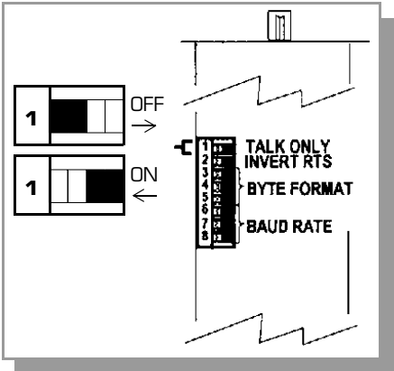
Figure 2-13 Partial Top View of RS-232 Module.
