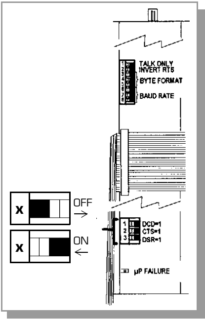
Figure 2-14 Top View of RS-232 Module.
