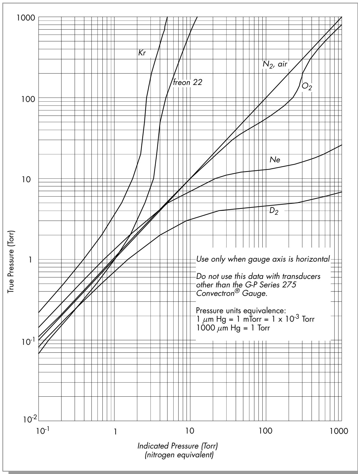
Figure 4-11 Convector Gauge Indicated vs. True Pressure Curve; 10^{-1} to 1000 Torr.
