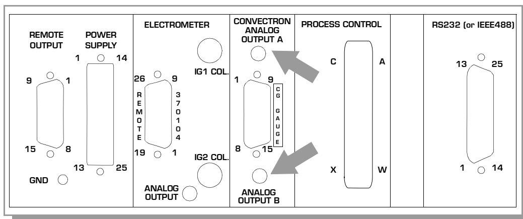
Figure 3-6 Convectron Gauge Analog Output Connector Locations on Rear Panel of Control Unit.
