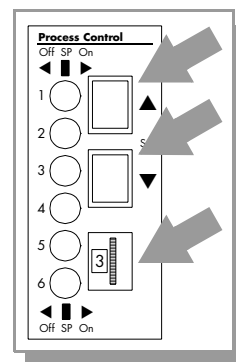
Figure 4-19 Electrometer Module Showing Setpoint Set Buttons and Channel Select Thumbwheel.
