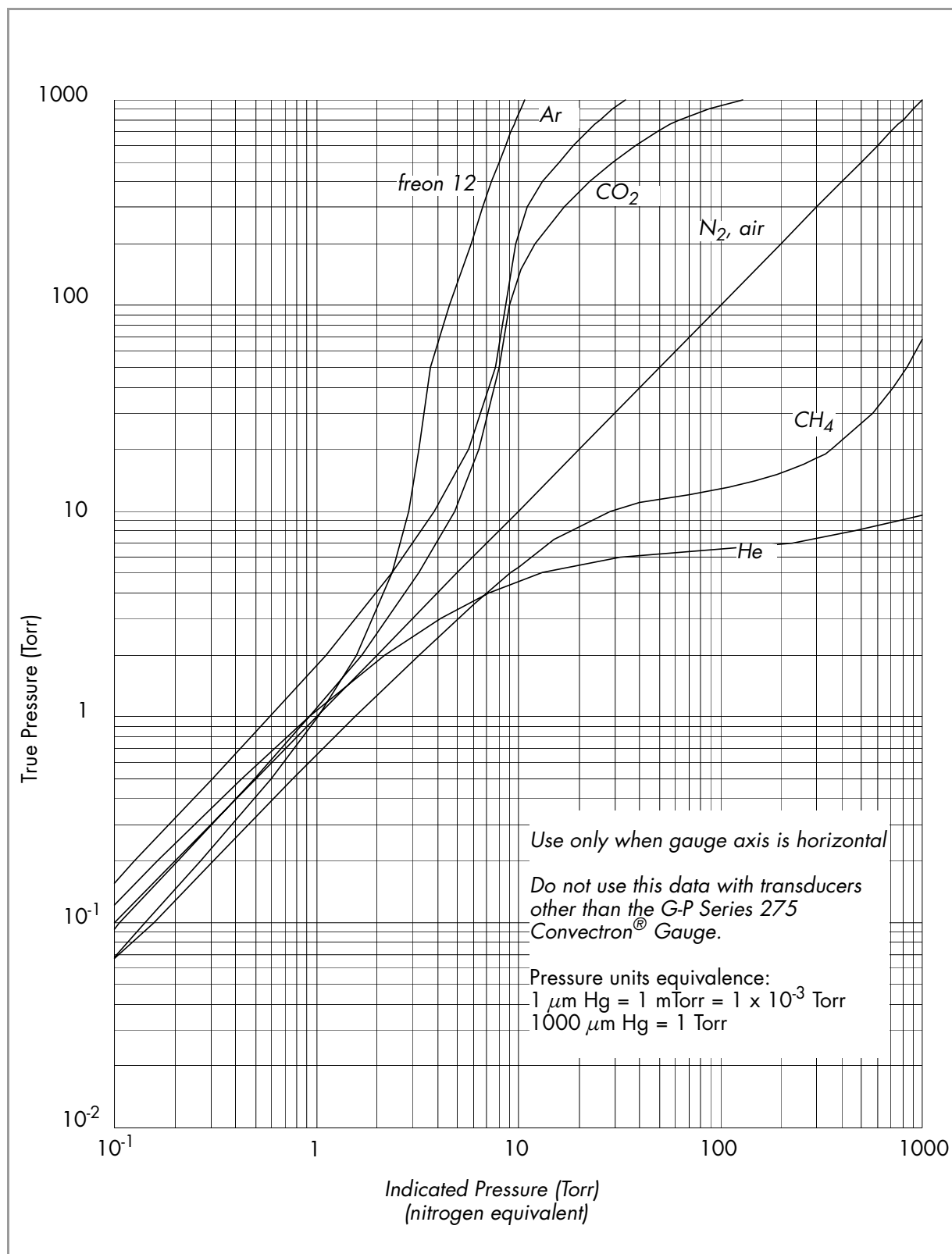
Figure 4-10 Convectron Gauge Indicated vs. True Pressure Curve; 10^{-1} to 1000 Torr.
