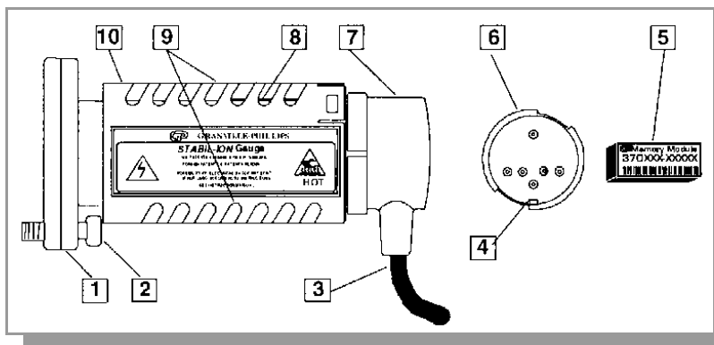
Figure 1-2 Stabil-Ion Gauge.
