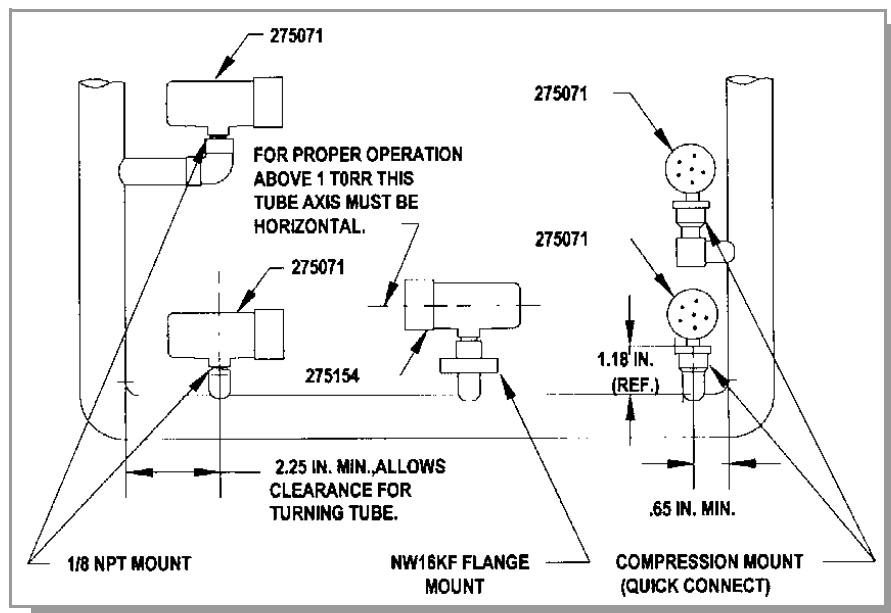
Figure 3-3 Convectron Gauge Installation.
