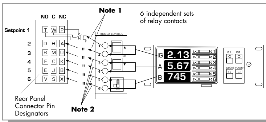
Figure 2-7 Six Channel Process Control - Cat. No. 370107.
