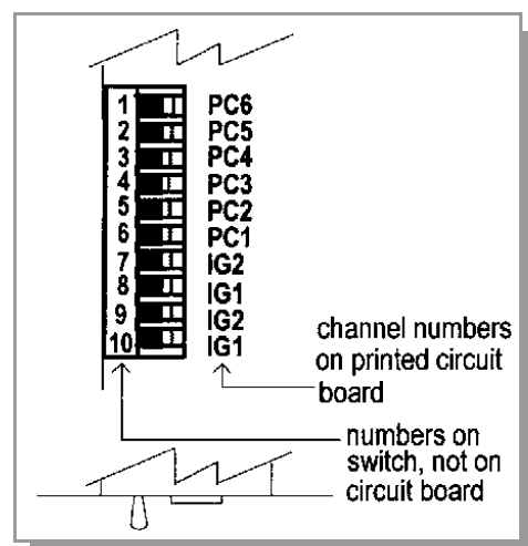
Figure 2-10 Partial Top View of Process Control Module.
