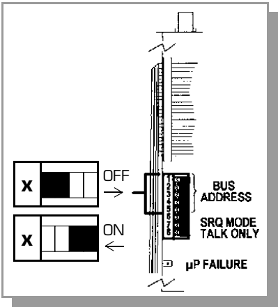
Figure 2-16 Top View of IEEE 488 Module.
