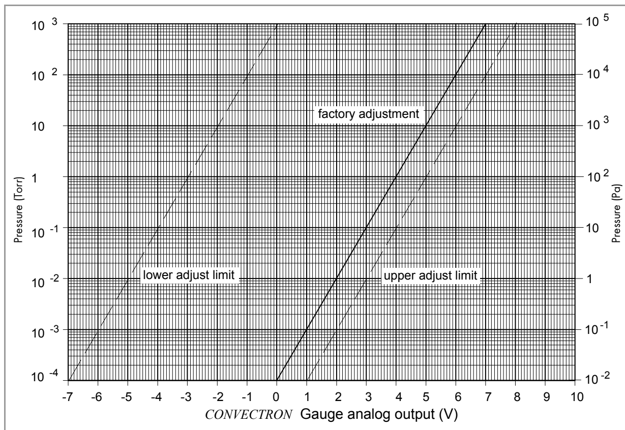
Figure 4-18 Convectron Gauge Analog Output vs. Pressure.
