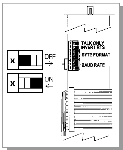
Figure 2-11 Partial Top View of Process Control Module.
