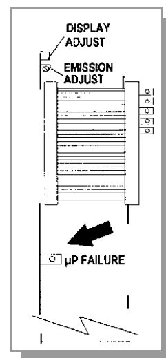
Figure 6-4 Electrometer Module, Top View Showing μP Failure LED.
