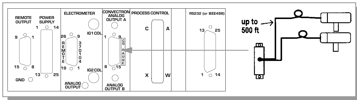
Figure 3-13 Control Unit Rear Panel Showing the Cable Connection to the Convector Gauges.
