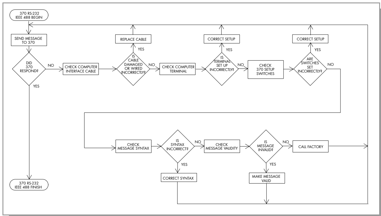
Figure 6-10 RS-232/IEEE 488 Interface.
