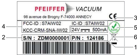
Fig. 1: Nameplate example
