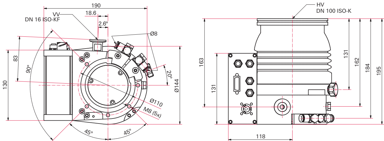
Fig. 24: Dimensions HiPace 300 | TC 400 | DN 100 ISO-K
