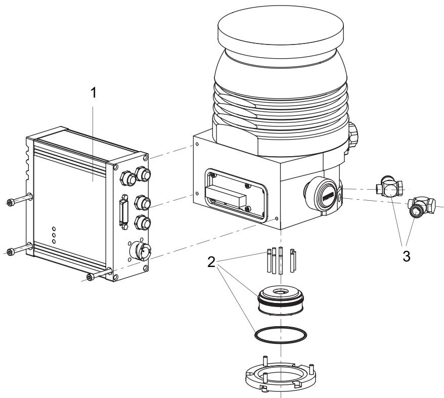
Fig. 23: Spare parts HiPace 300
