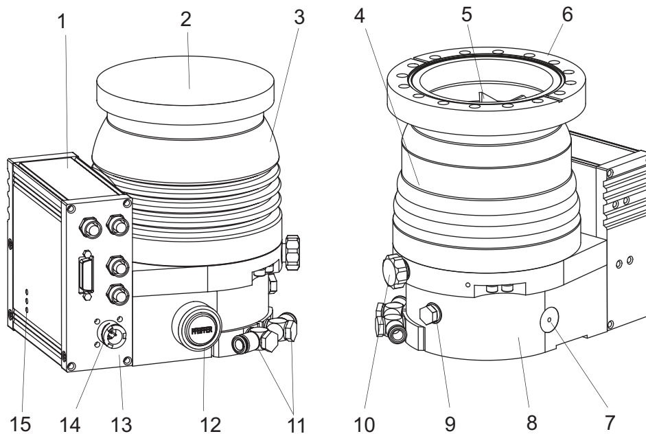
Fig. 3: HiPace 300 design
