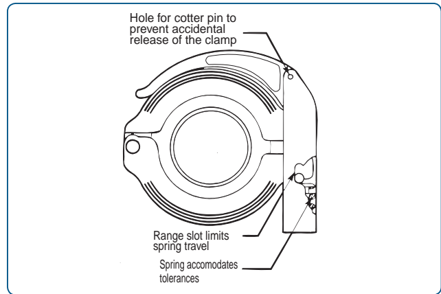
Figure 3 — Toggle Clamp
