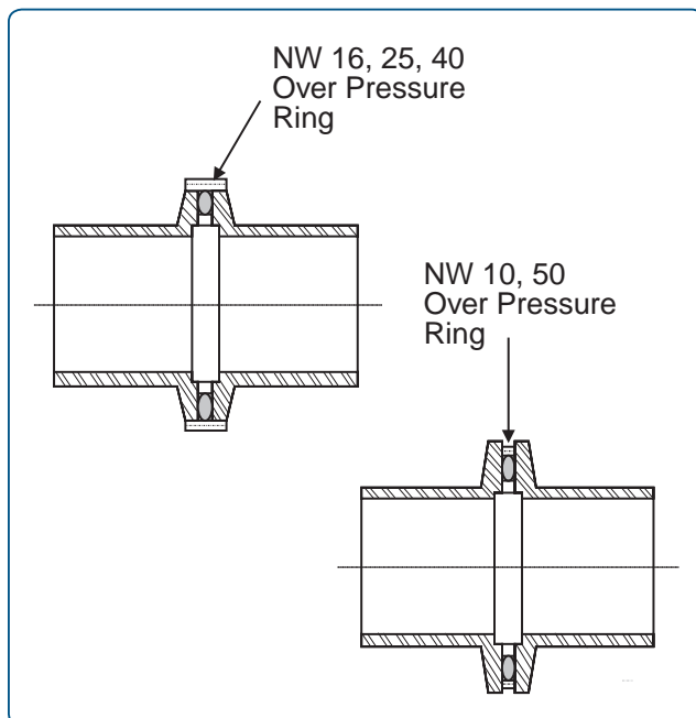
Figure 6 — Overpressure Rings
