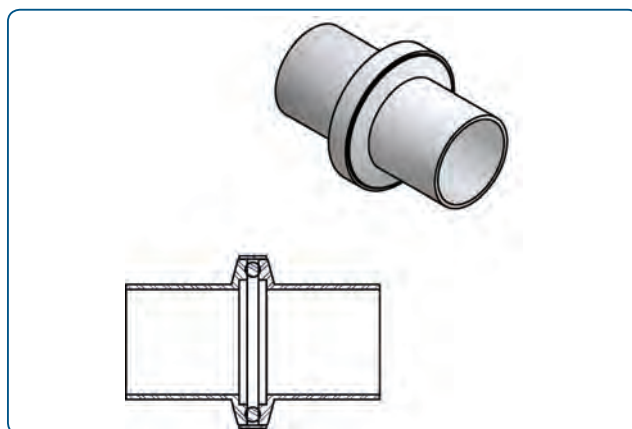
Figure 6a — Captured O-Ring Overpressure Assembly
