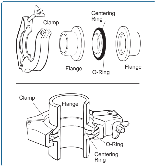
Figure 2 — Component Assembly
