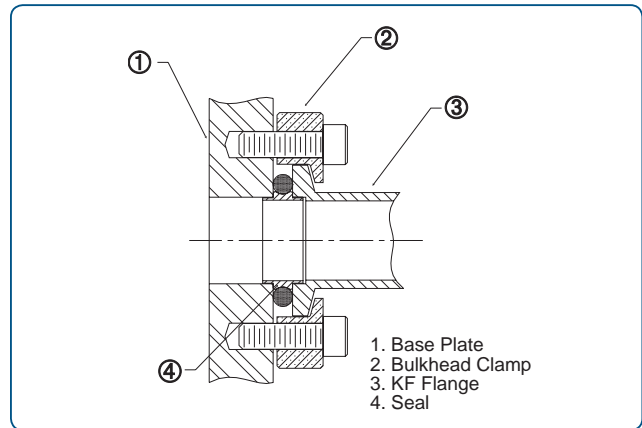
Figure 4 — Bulkhead Clamp
