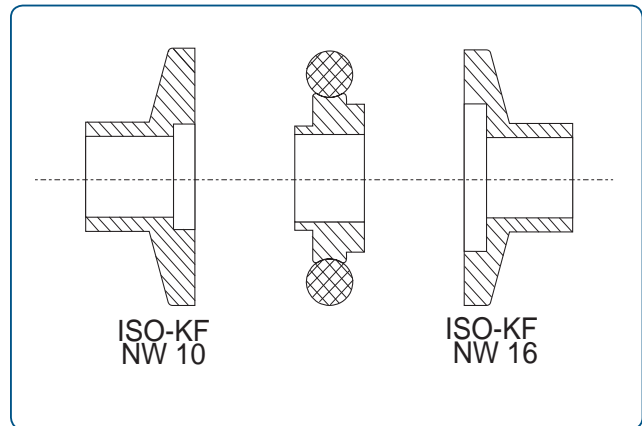
Figure 5 — Adaptive Centering Rings
