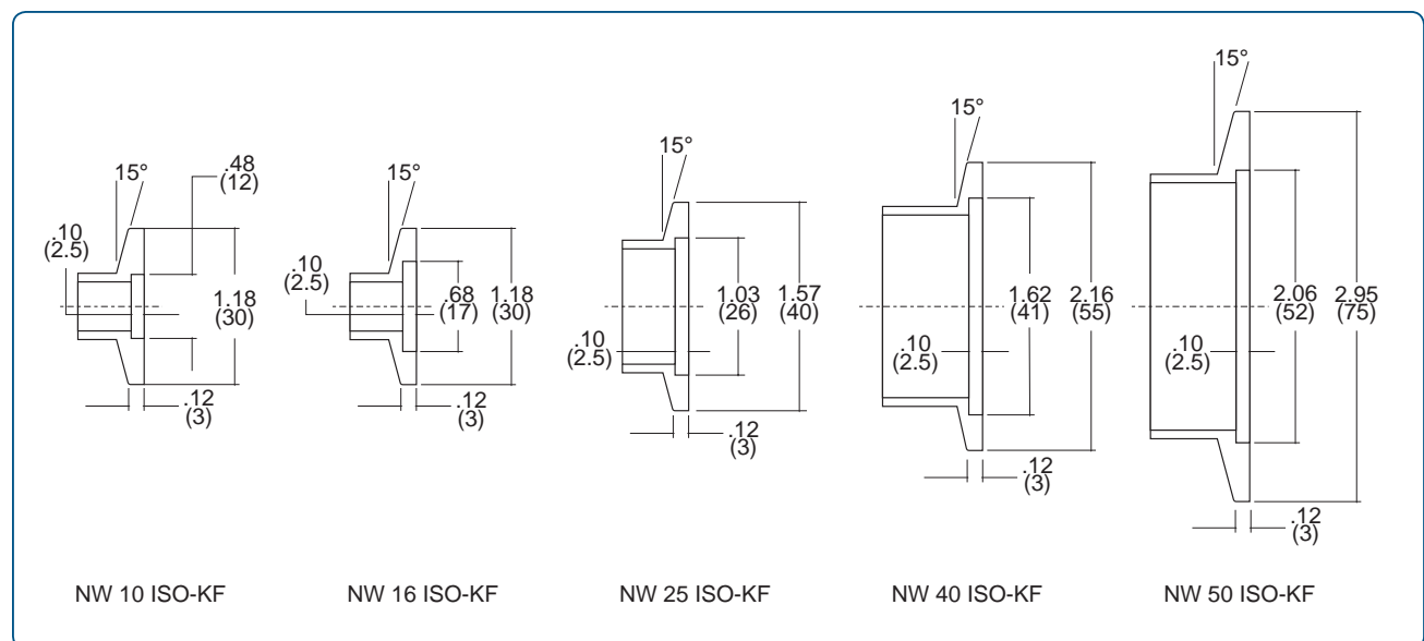
Figure 1 — ISO-KF Flange Dimensions
