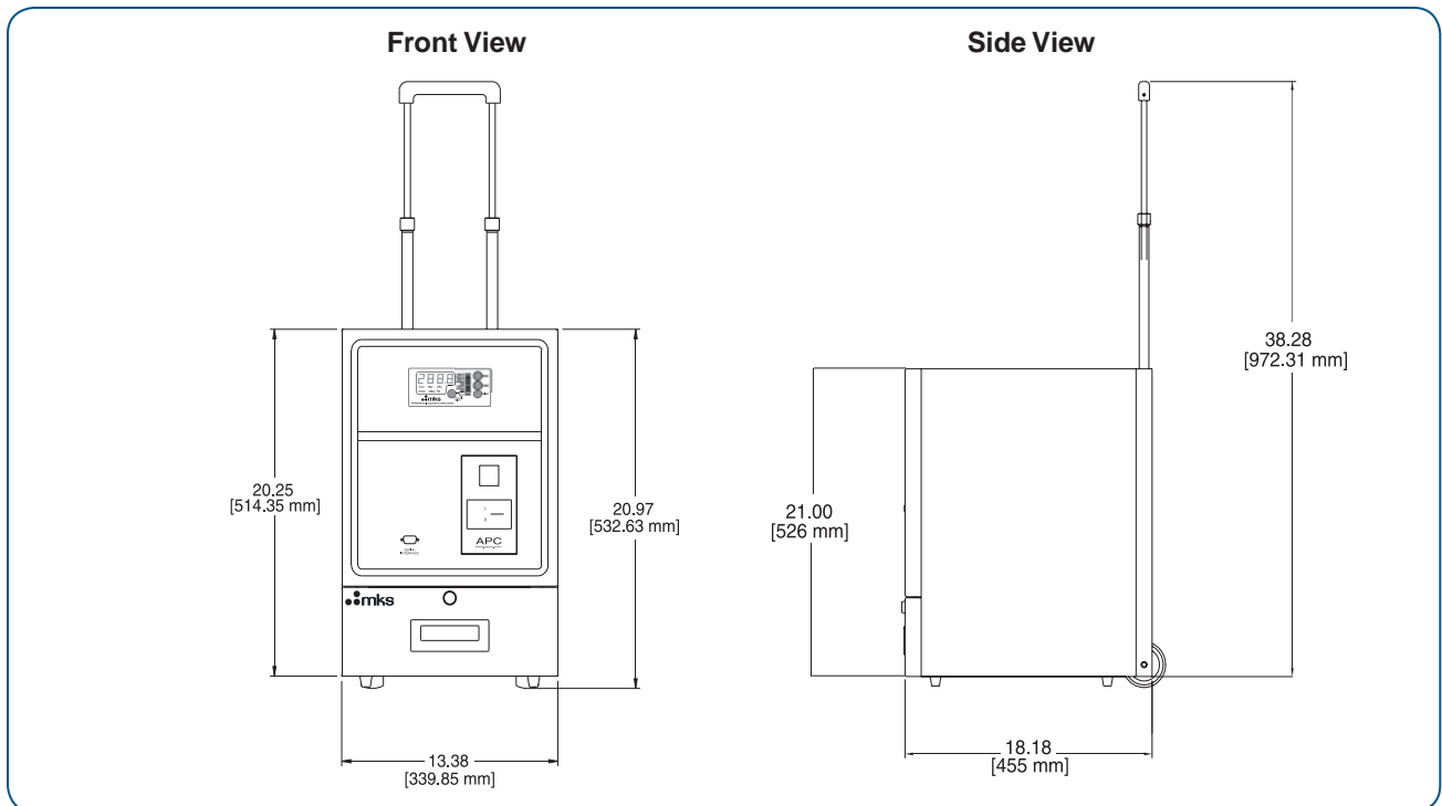
Dimensional Drawing — Note: Unless otherwise specified, dimensions are nominal values in inches (mm referenced).
