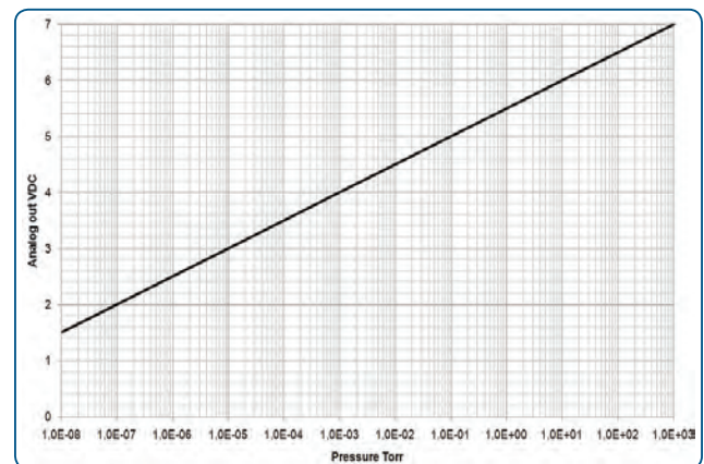
Analog Output
