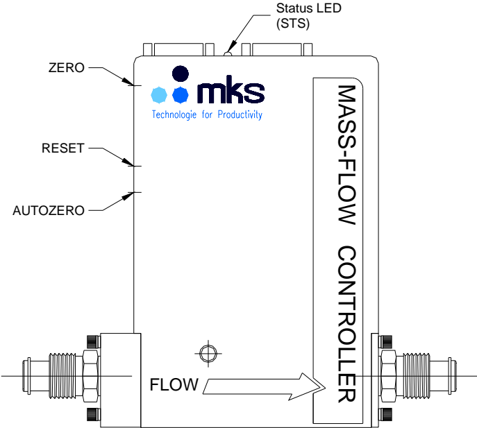
Figure 6: 1579A/B / 579A/B Side View (Imprint on type 579A/B: MASS-FLOW METER )
