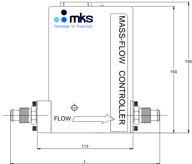
Figure 11: 1579A/B / 579A/B Dimensions (Side)
