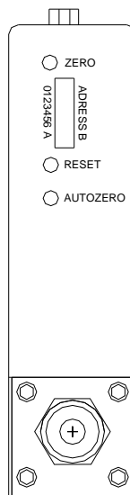
Figure 8: 1579A/B / 579A/B Gas Inlet Side
