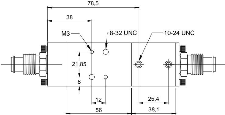
Figure 13: Mounting Holes
