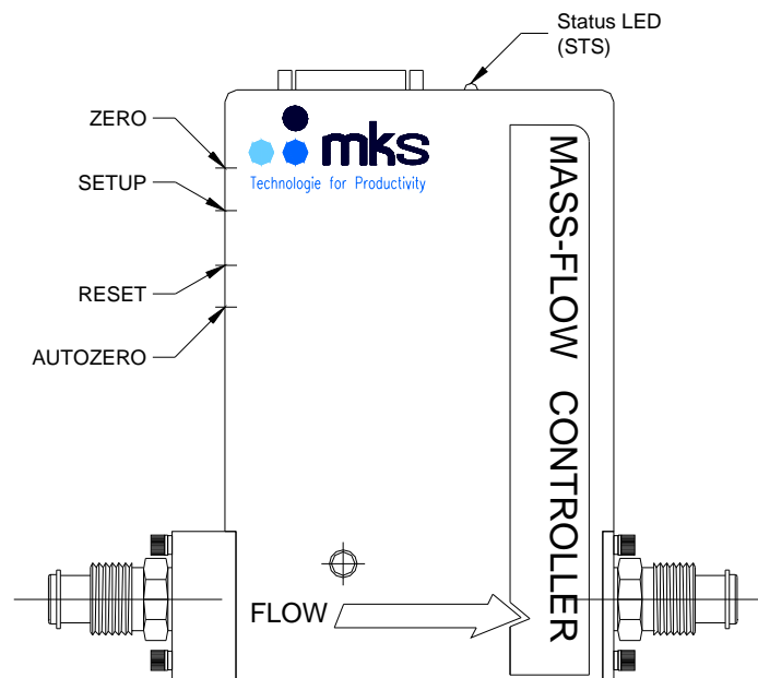
Figure 2: 1579A/B / 579A/B Side View (Imprint on type 579A/B: MASS-FLOW METER )
