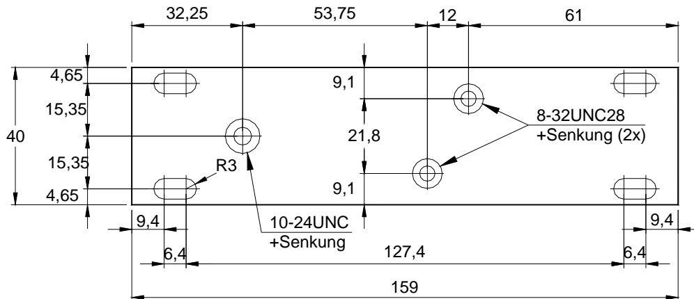
Figure 14: Mounting Plate
