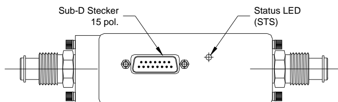
Figure 3: 1579A/B / 579A/B Connector Side
