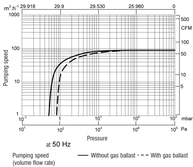
Pumping speeds curves SV100 B
