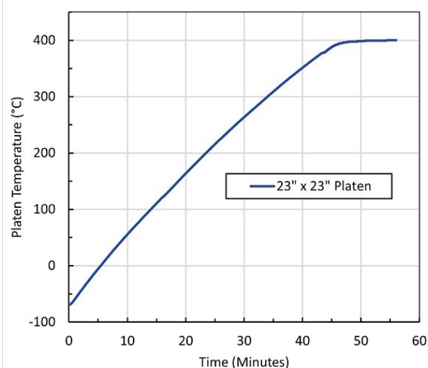
Platen heating temp. vs. time
