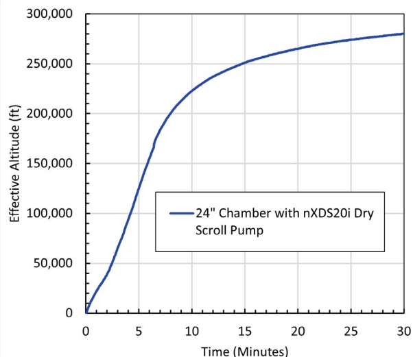
Effective altitude vs. time
