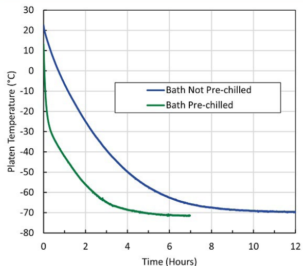
Platen cooling vs. time
