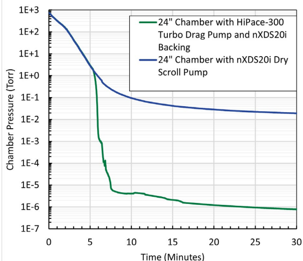
Chamber pressure vs. time
