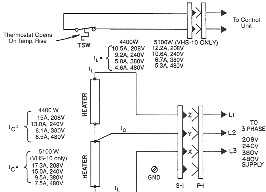
Figure 1-4 Operating Characteristics
