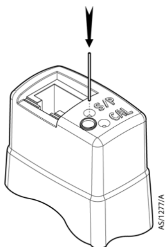
Figure 9 - Adjusting set-point
