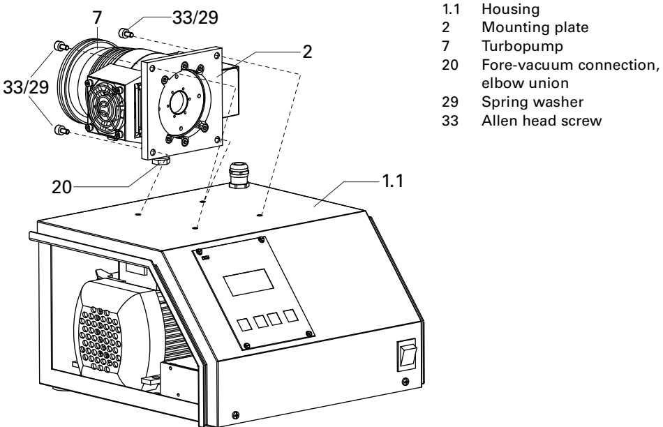
Fig. 6: Disassembly of the turbopump
