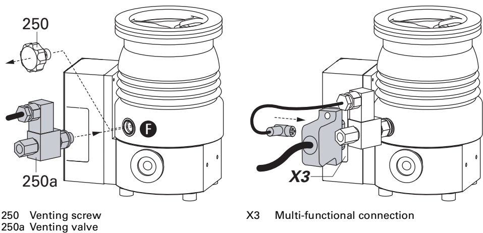
Fig. 9: Connecting the venting valve
