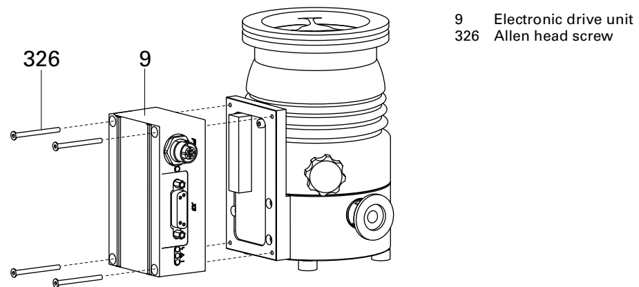
Fig. 16: Assembly / disassembly of the TC 110
