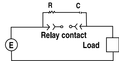
Relay arc suppression network
