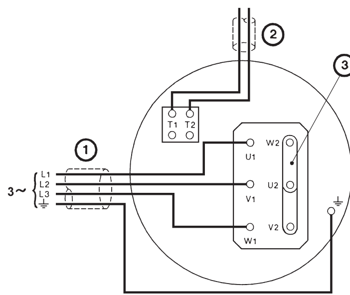
Figure 12 - QMB250/500F low-voltage configuration
