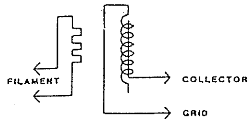
Fig. 1.15 Ion Gauge Schematic
