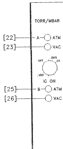
Fig. 5.12 Convectron Module Front Panel
