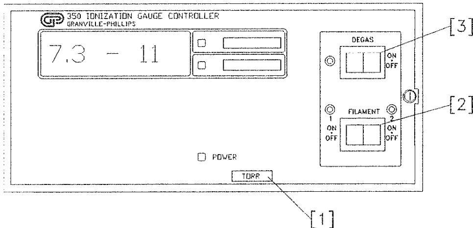
Fig. 1.12 350 IGC Control Unit Front Panel
