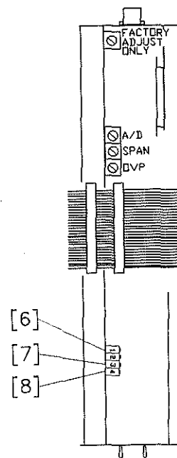
Fig. 2.1 Ion Gauge Electrometer Module Top View
