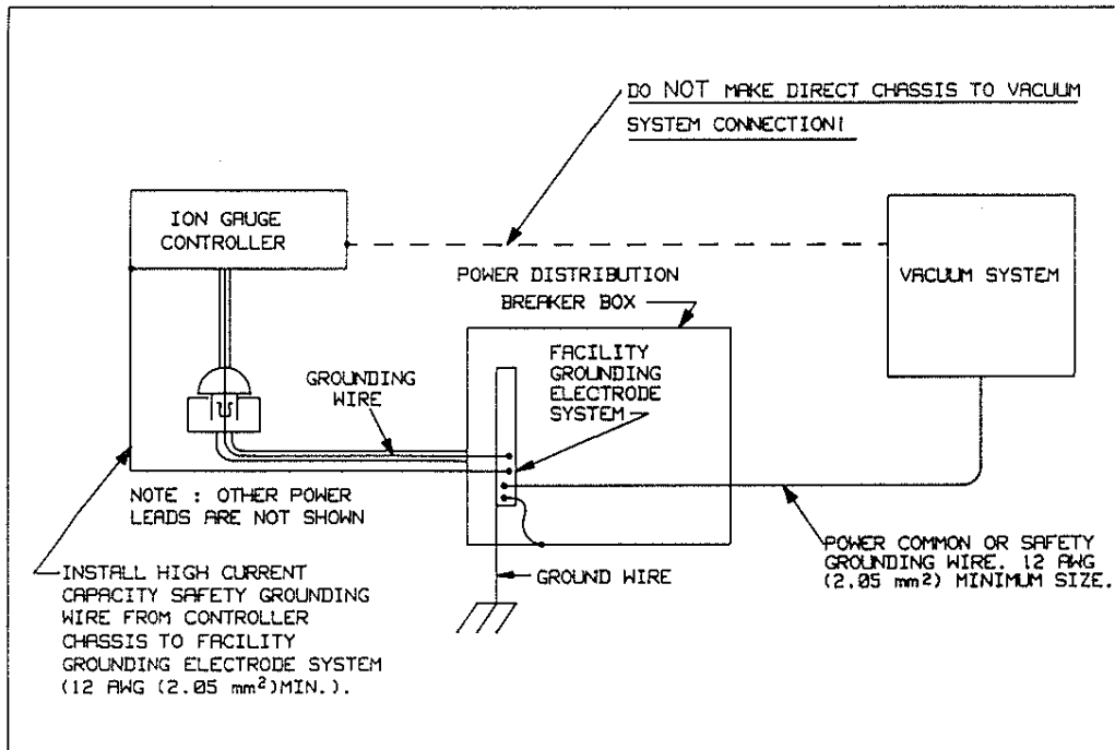
Fig. 1.11 Correct System Grounding
