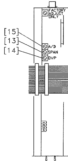
Fig. 2.5 Ion Gauge Electrometer Module
