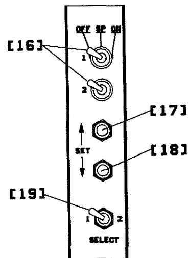
Fig. 3.1 Process Control Module, Front Panel
