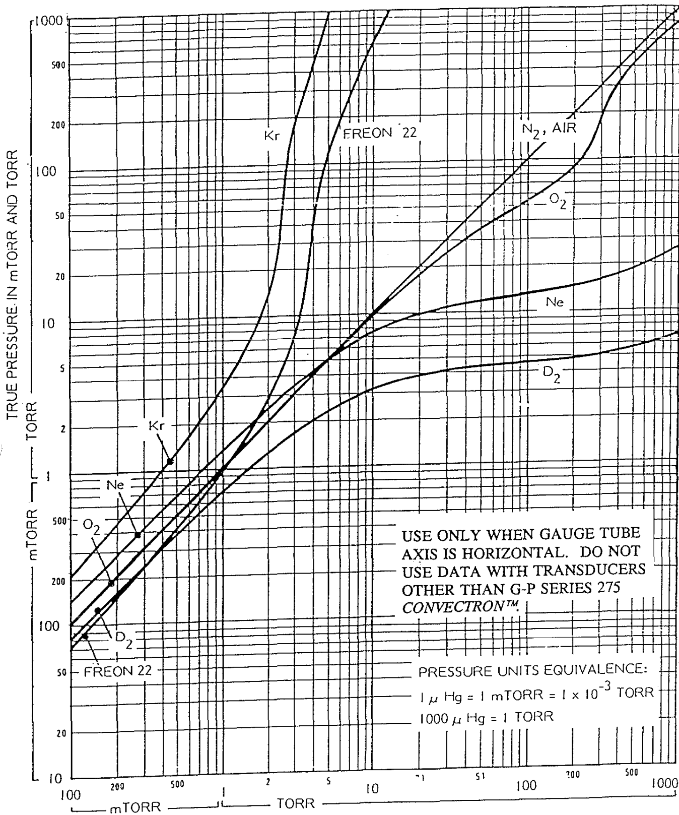
INDICATED PRESSURE IN mTORR AND TORR (N 2 EQUIVALENT)
