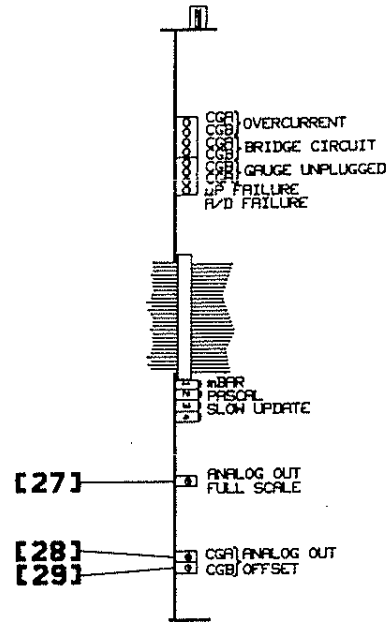
Fig. 5.11 Convectron Module Top View
