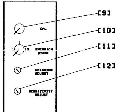
Fig. 2.2 Electrometer Module Front Panel
