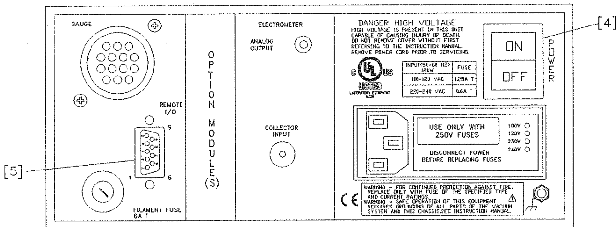
Fig. 1.13 350 IGC Control Unit Rear Panel
