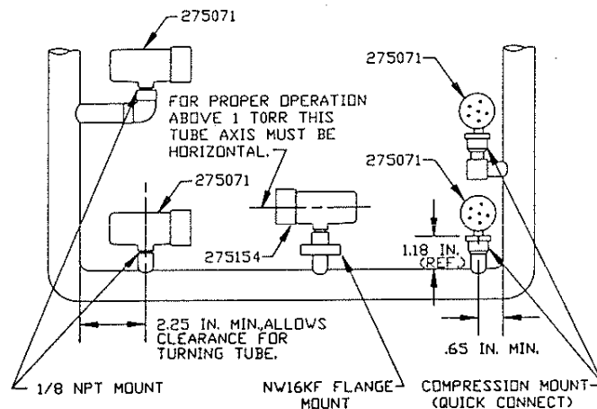
Fig. 5.2 Convectron Gauge Mounting
