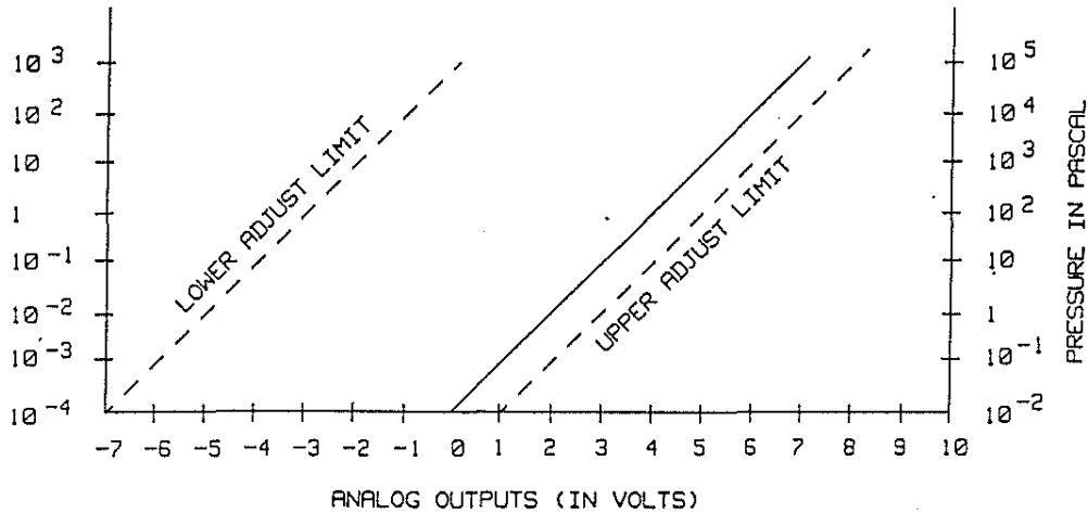
Fig. 5.10 Convectron Gauge Pressure Analog Output
