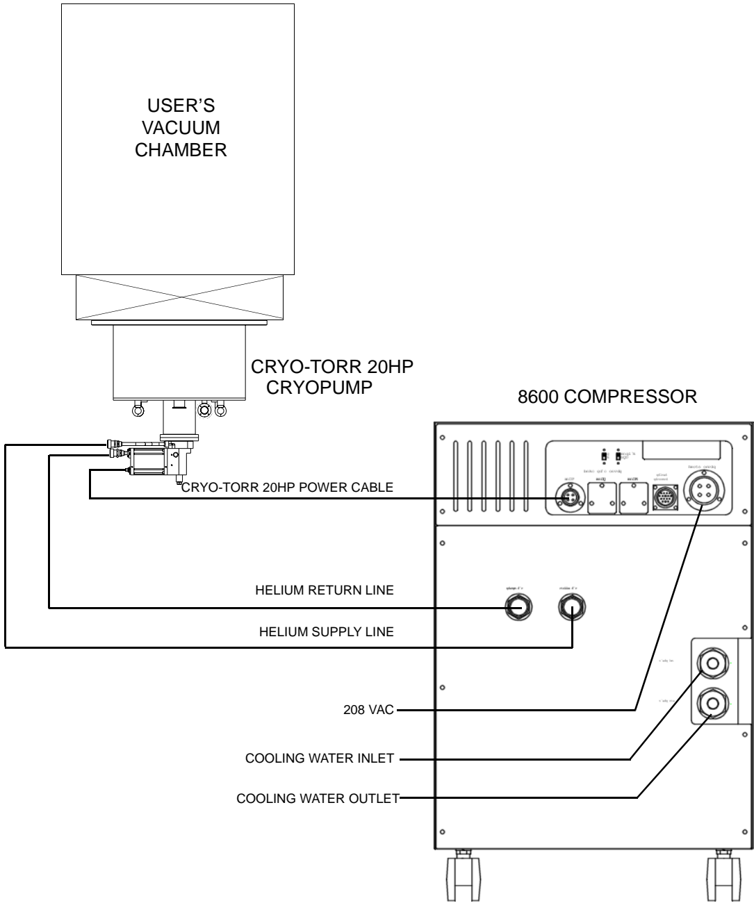
Figure 1-7: Typical Cryo-Torr System with 8600 Compressor
