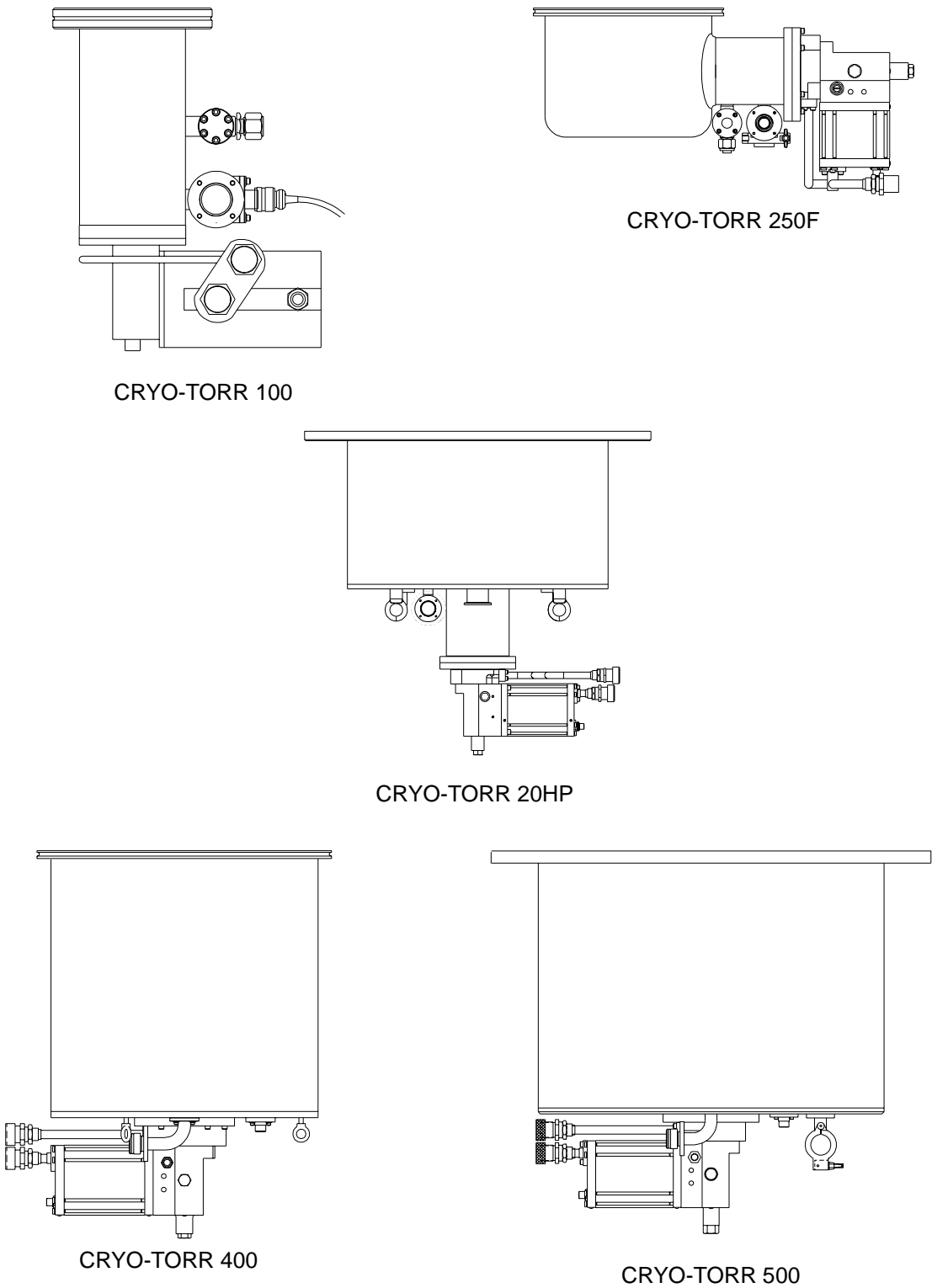
Figure 1-2: Cryo-Torr Pumps
