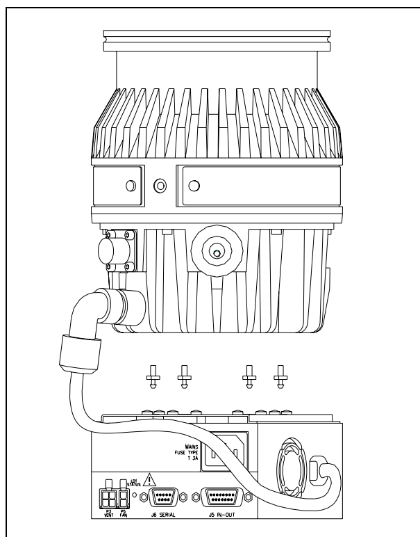
MOUNTING 1
