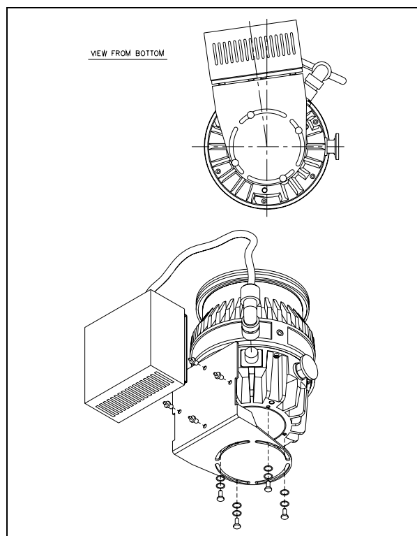
MOUNTING 2
